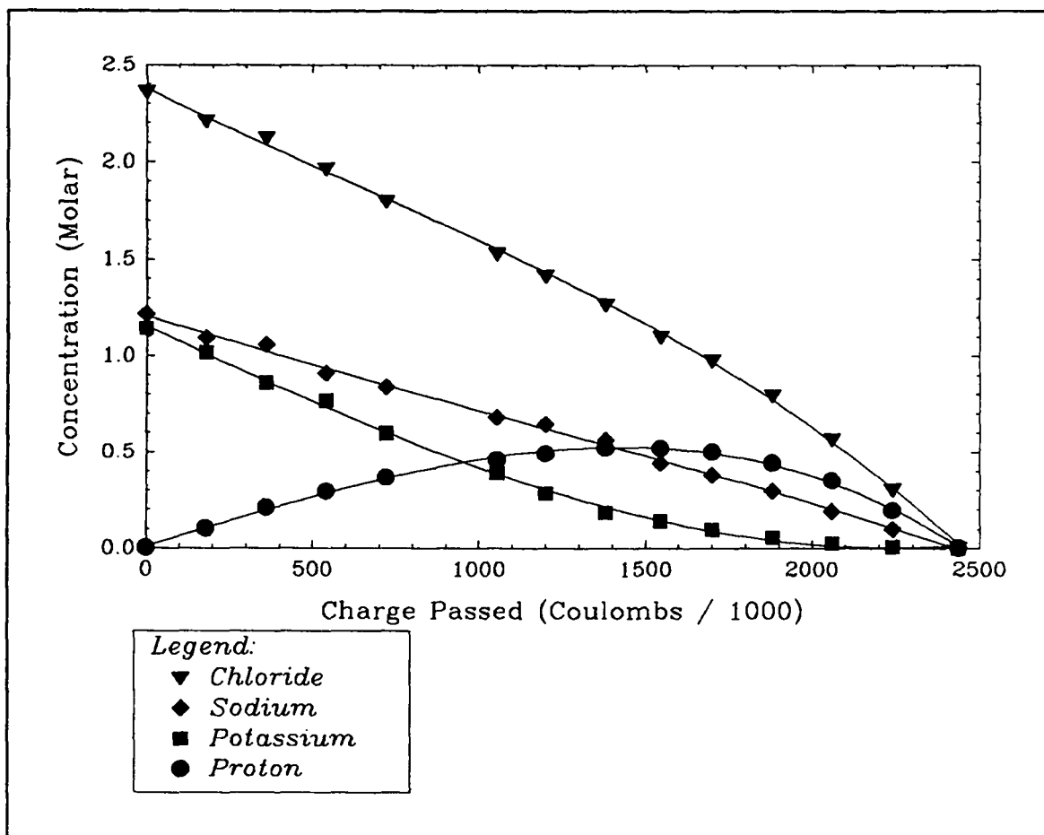
Figure 10: Concentration changes in the feed solution during the stage two electrodiagnosis.
