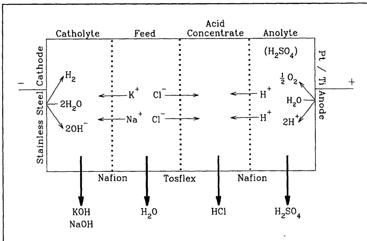
Figure 5: Diagram of a four-compartment electrodiagnosis cell for the second electrodiagnosis stage.
