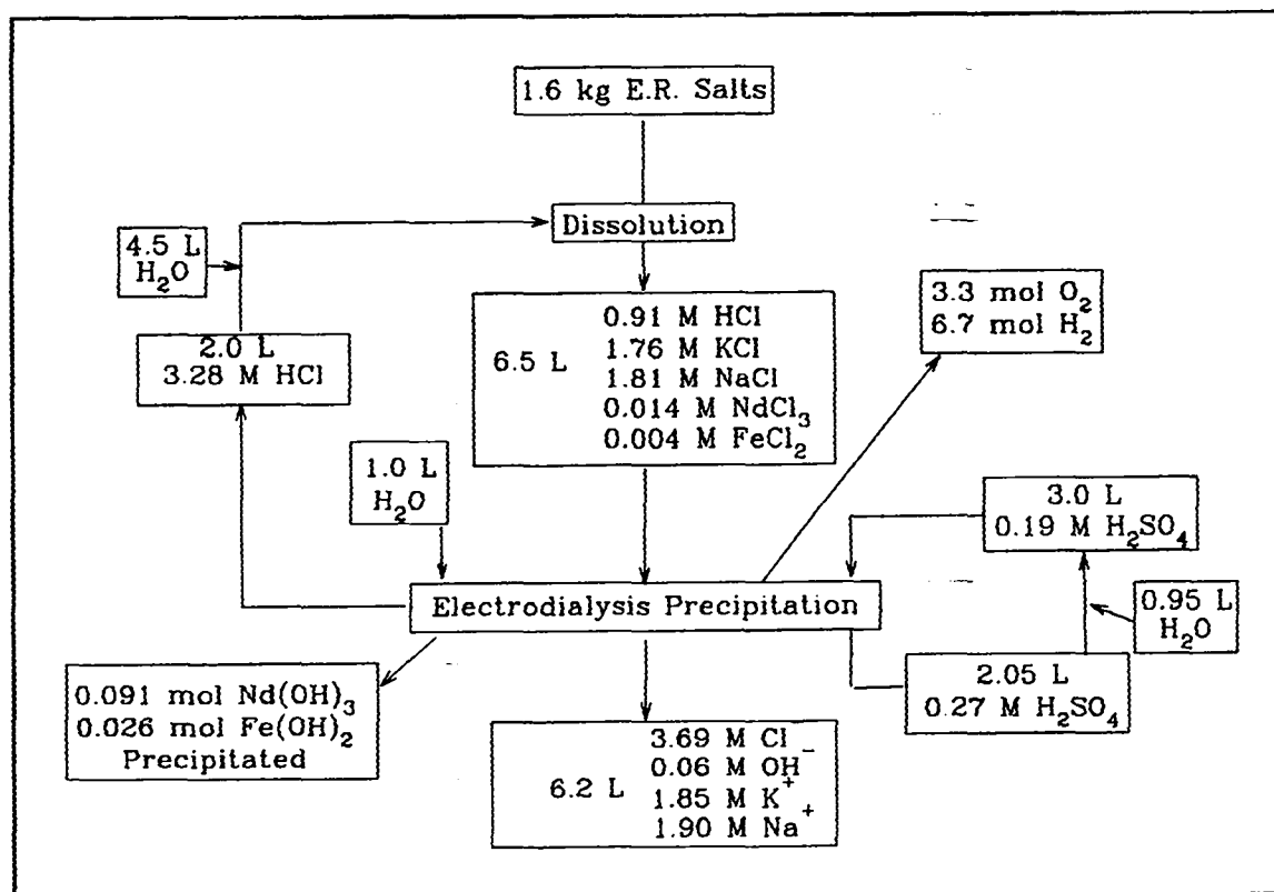
Figure 9: Mass balances for first stage electrodiolysis.
